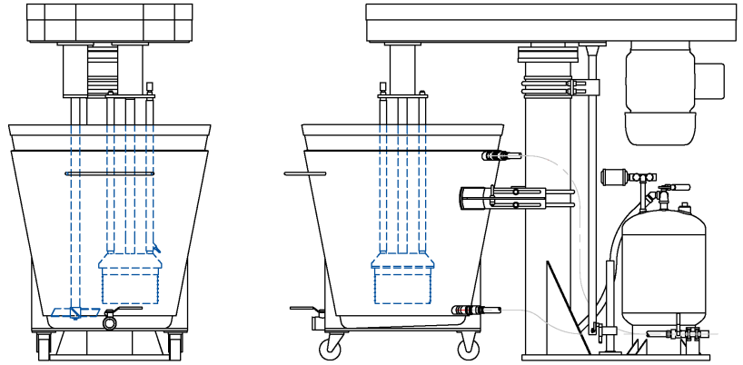
Dimensional Drawing Batch Mill with Tank Refer to Chart for Dimensions
